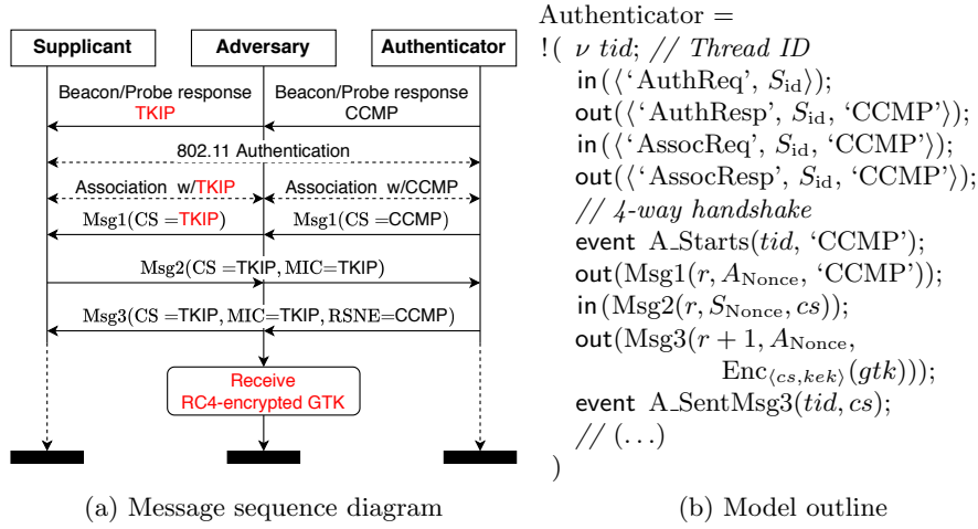
Fig. 9: Downgrade Attack on 802.11 (TP-Link WP841P)
